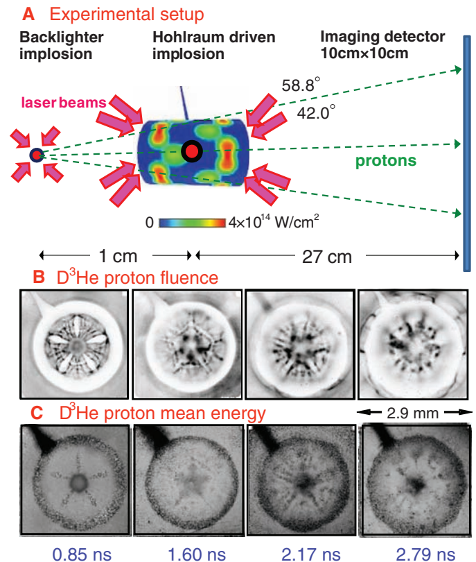
Fig. 1. (A) Schematic of the experimental setup, with proton backlighter, hohlraum-driven implosion, CR-39 imaging detector, and laser drive beams. Fifteen laser beams entered each end of the hohlraum: 5 with incident angle 42° and 10 with angle 58.8°. The colors shown on the hohlraum wall indicate the laser intensity distribution [modeled by VISRAD (26)]. The proton backlighter was driven by 30 laser beams with total laser energy \sim 11 \text{ kJ} in a 1-ns square pulse. The 15 MeV \text{D}^3\text{He} backlighting protons (16) passed through the laser-driven hohlraum, sampling plasma conditions, and capsule implosions at different times. Images in (B) show proton fluence (within each image, darker means higher fluence), whereas images in (C) show proton energy (within each image, darker means more proton energy loss and therefore more matter traversed). The grayscale mapping for image display is different in each image. The hohlraum-mounting stalk appears in the upper left corner of each image.
